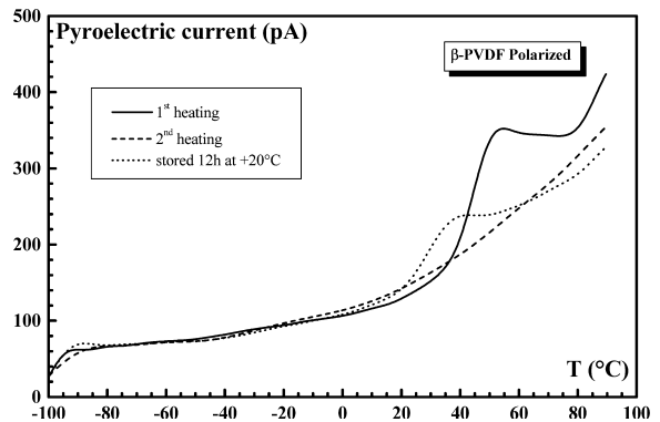
Fig. 2. Evolution of the pyroelectric current upon temperature for poled \beta -form PVDF (experimental conditions and annealing procedures are given in the text).
