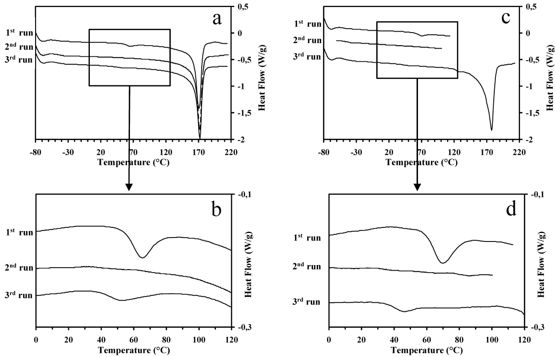
Fig. 1. DSC traces of (a,b) \alpha -form PVDF and (c,d) \beta -form PVDF. The first run is immediately followed by the second run, whereas an annealing at room temperature for 5 h takes place before the third run (see text for details).
