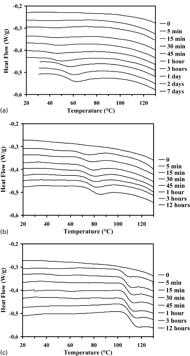
Fig. 4. DSC traces of \alpha -form PVDF after annealing for various times at (a) T = 23 °C, (b) T = 60 °C, (c) T = 100 °C. The annealing time is indicated next to each trace.
