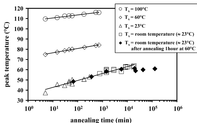
Fig. 5. Plot of the DSC annealing-peak temperature ( T_m^{\text{low}} ) as a function of annealing time ( t_x ) for \alpha -form PVDF. For each annealing temperature T_x , the line corresponds to the best fit obtained with Eq. (3). The parameters resulting from the fit are given in Table 1.
