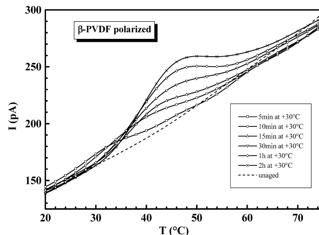
Fig. 6. Evolution of the TSC annealing-peak for poled \beta -form PVDF samples annealed for various times at +30^\circ\text{C} .
